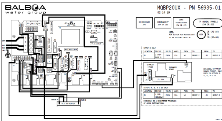
Wiring Diagram
